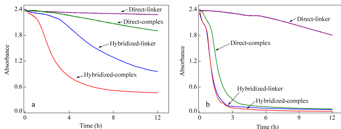
Fig. 4 Comparison of the kinetics for assembly of DNA-AuNPs in linker-addition and DNA-machine-driven strategies at different molar ratios of [\text{linker or complex}]/[\text{AuNPs}] : (a) [\text{linker or complex}]/[\text{AuNPs}] = 10 and (b) [\text{linker or complex}]/[\text{AuNPs}] = 21 .
