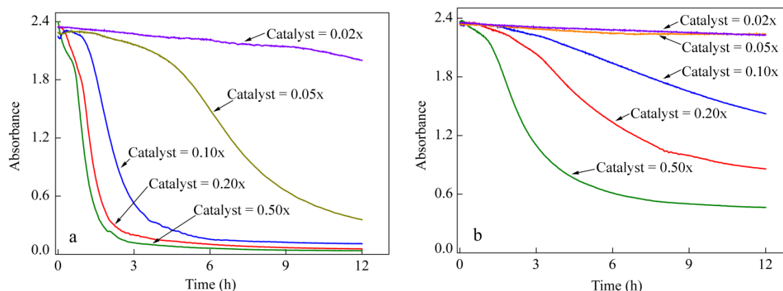
Fig. 3 Dependence of the kinetics of the assembly of DNA-AuNPs using the hybridized-complex-addition strategy on catalyst-oligonucleotide concentrations at different molar ratios of [\text{complex}]/[\text{AuNPs}] : (a) [\text{complex}]/[\text{AuNPs}] = 21 and (b) [\text{complex}]/[\text{AuNPs}] = 10 . The amount of catalyst-oligonucleotide changed with various coefficient according to the amount of complex used in different systems.
